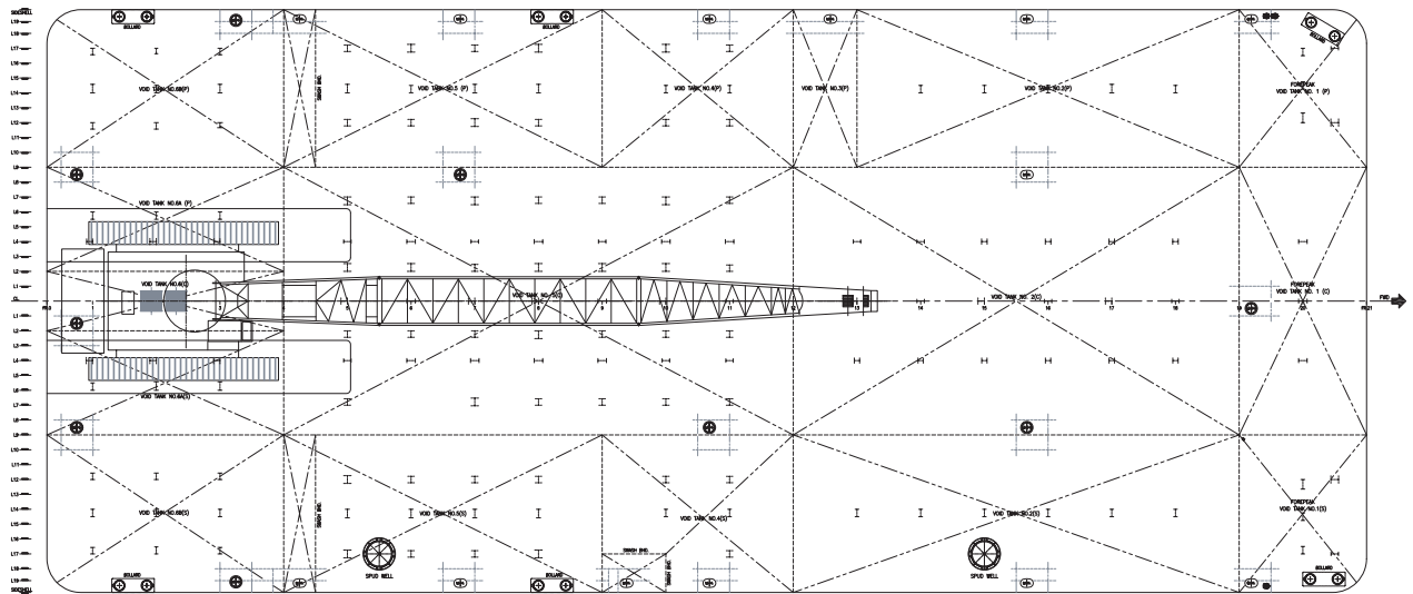
Below main deck/tank plan
