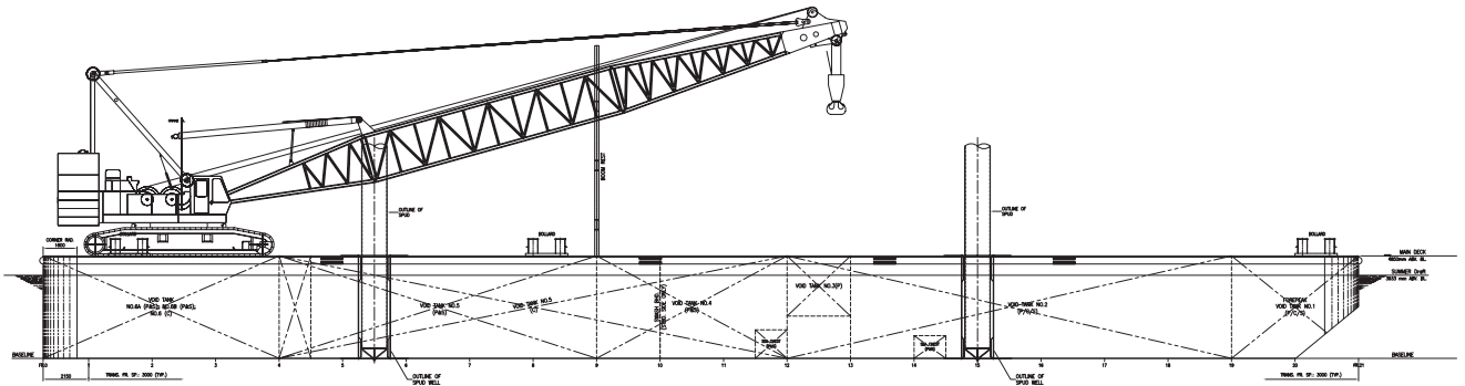
Outboard profile
